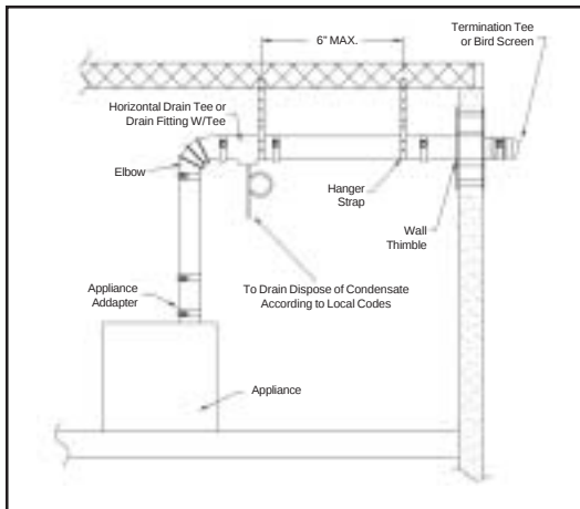
Side Wall Installation
