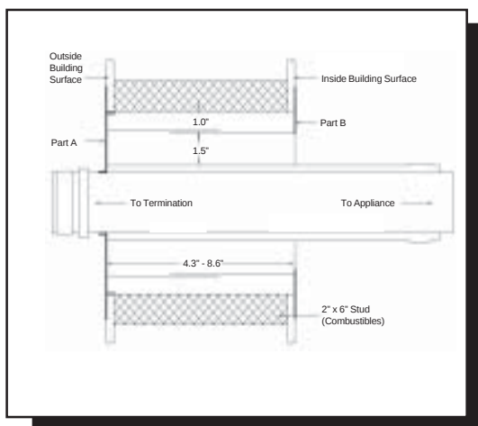
Wall Thimble Installation
